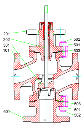
MV 5221, PV 6221, DN 20-80; 1"-3", PN 16-40; #150/300
