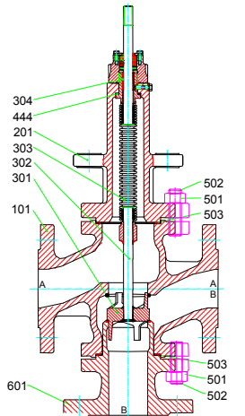
MV 5221, PV 6221, DN 80-100; 3"-4", PN 16-40; #150/300
