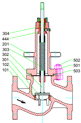
MV 5211, PV 6211, DN 80-100; 3"-4", PN 16-40; #150/300
