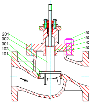
MV 5211, PV 6211, DN 15-65; 1"-2 1/2", PN 16-40; #150/300
