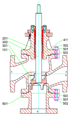
MV 5421, PV 6421, DN 80-400; 3"-12", PN 16-40; #150/300
