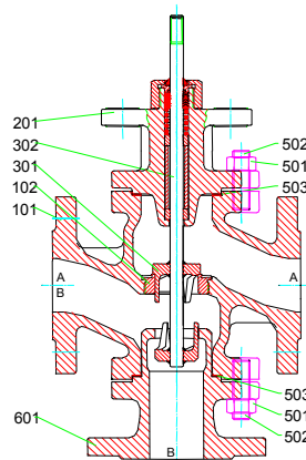
MV 5231, PV 6231, DN 20-80; 1"-3", PN 16-40; #150/300
