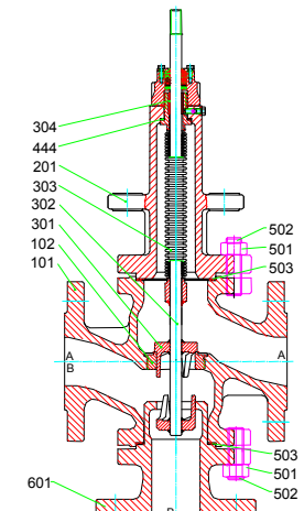
MV 5231, PV 6231, DN 80-100; 3"-4", PN 16-40; #150/300
