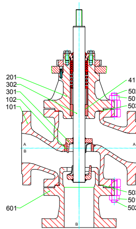
MV 5431, PV 6431, DN 80-400; 3"-10", PN 16-40; #150/300
