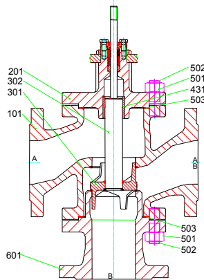
MV 5221, PV 6221, DN 20-80; 1"-3", PN 16-40; #150/300
